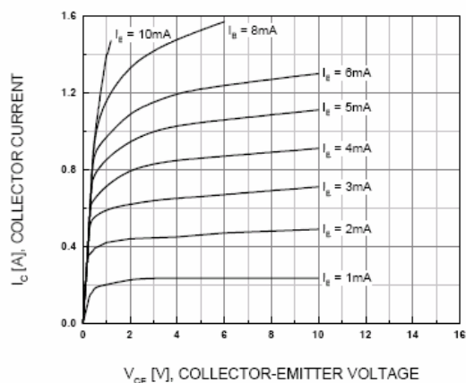
Figure 1. Static Characteristics
